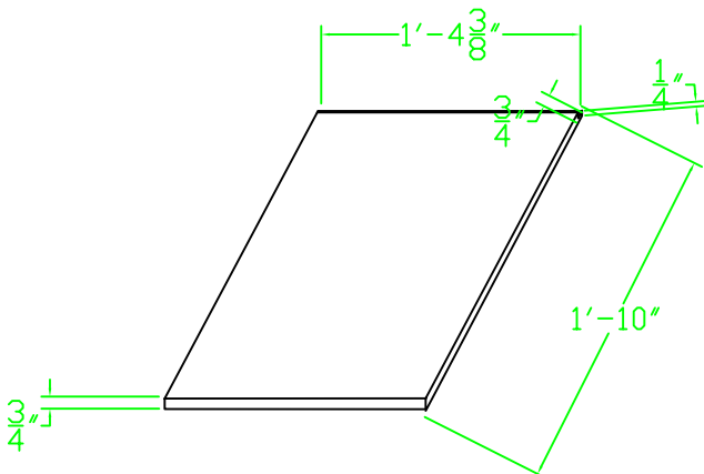
COVER 16 3/8 INCHES X 22 INCHES SECURES TO SIDES, BACK END, AND FRONT ENTRANCE PANELS
