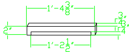
FRONT ENTRANCE PANEL QTY 1 2 INCHES X 16 3/8 INCHES CUT OUT NOTCH 14 1/2 INCHES X 3/4 OF AN INCH FOR ENTRANCE REDUCER SECURES TO COVER AND SIDE PANELS
