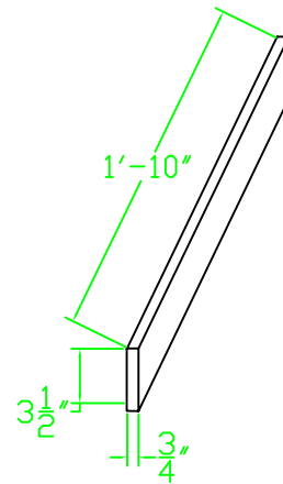
SIDE PANELS QTY 2 3 1/2 INCHES X 22 INCHES SECURES TO COVER, FRONT ENTRANCE, LANDING, AND BACK END PANELS.
