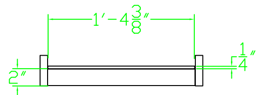
SIDE VIEW WITH CUT AWAY SHOWN RESTING ON HIVE BOX
