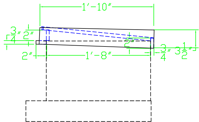
SIDE VIEW WITH CUT AWAY SHOWN RESTING ON HIVE BOX
